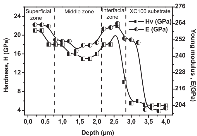
Fig. 10. Hardness and Young's modulus of the CrN coatings, annealed at 900 °C, as a function of the penetration depth.
